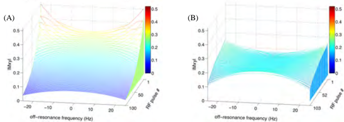
Figure 2. Bloch simulation results of bSSFP transient state signal profile as a function of off-resonance frequency and number of echoes for CFA (A) and VFA (B) schemes.
