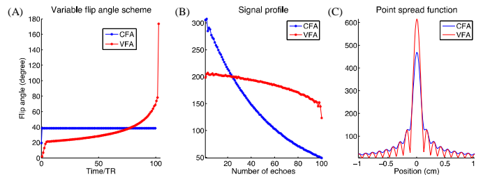
Figure 1. Flip angle scheme (A) for bSSFP sequence including constant flip angle (CFA) and variable flip angle (VFA). The signal profile (B) and the corresponding point spread function (C) were measured for spins on resonance.
