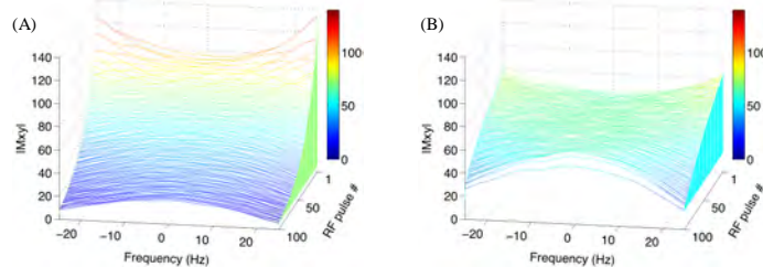
Figure 3. Measured signal profiles as in Figure 2.
