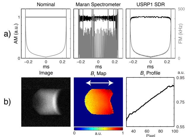
Figure 3. (a) Comparison of nominal and measured frequency-swept pulses generated by the Maran spectrometer and the USRP1 SDR. (b) Image, Bloch-Siegert B_1 map and B_1 profile (averaged across length indicated by white line) in a water phantom using the USRP1 for all RF excitation pulses.
