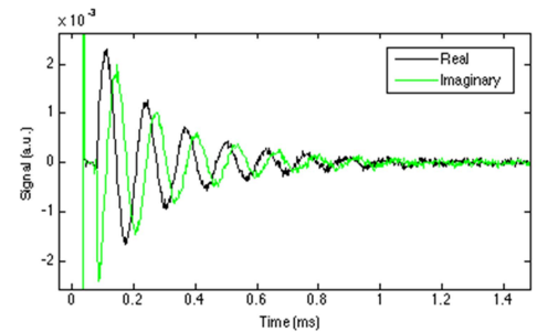
Figure 2: A pulse-and-acquire FID recorded by the USRP1.
