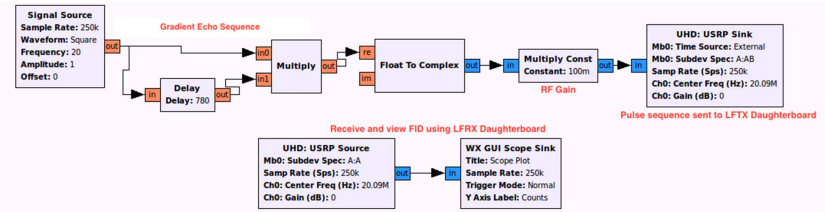
Figure 1: GNURadio block diagram for a pulse-and-acquire FID experiment.
