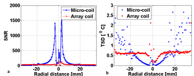
Fig. 3: a) SNR versus radius, b) temperature standard deviation
