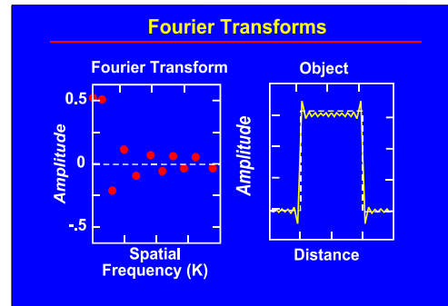
Figure 24. The K-space representation (left) of the Fourier components to create the target function (right).
