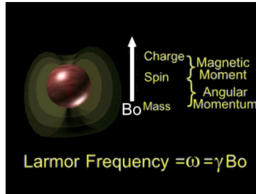
Figure 1. The precession of a proton in a magnetic field B_0 , arises from its charge, mass and spin.
