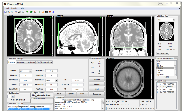
Figure 1. 3D-bSSFP simulation at 3.0T using MRiLab. Figure shows the main simulation panel and one axial slice of simulated bSSFP image. Note banding artifact is caused by added field variation.
