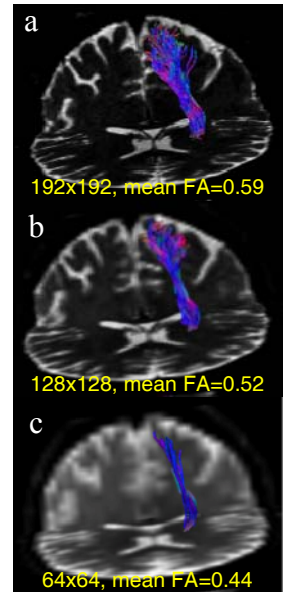
Fig.1 Reconstruction of the Cerebro-Spinal Tract (CST) at a) 1, b) 2 and c) 3mm isotropic
