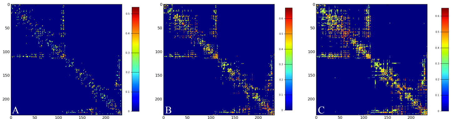
Fig.2 Matrices of mean FA between all pairs of n=234 ROIs respectively obtained for the (A) 3x3x3mm 3 , (B) 2x2x2mm 3 and (C) 1x1x1mm 3 datasets. The upper left and lower right blocks of the matrix respectively represent connections in the right and left hemisphere.
