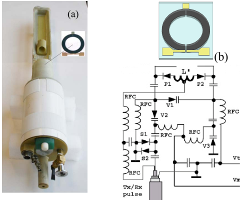
Figure 1. A picture of the liquid nitrogen 77 K G-10 cryostat with an animal bed attached (inset shows a picture of HTS coil) (a) and a sketch of the HS coil design connected to a high Q matching and tuning circuit (b) are shown. CC, P, and V denote coupling capacitors, PIN diodes, and varactor diodes (details are not shown).
