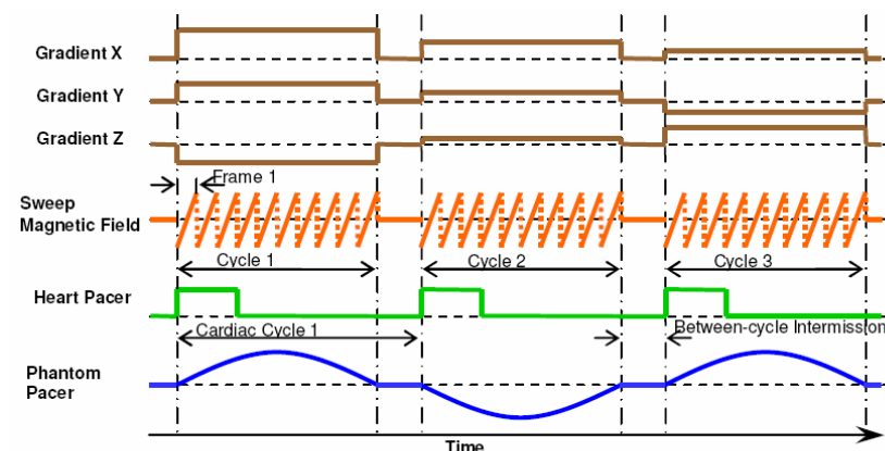
Fig. 1. Gradients, field sweep, and pacing waveforms for direct fast gated EPR acquisition
