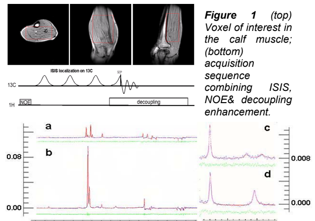
Figure 1 (top) Voxel of interest in the calf muscle; (bottom) acquisition sequence combining ISIS, NOE & decoupling enhancement. Figure 2 Calf muscle 13C spectra (blue), fitting (red) and residual (green): (a), direct acquisition; (b), with NOE and proton decoupling; (c), spectra from (a) enlarged 90-120ppm; (d), spectra from (b) enlarged 90-120ppm. (a) and (b), (c) and (d) are on the same scale, respectively. The ERETIC reference appears at 115ppm, glycogen peaks are centered at 100.5ppm.
