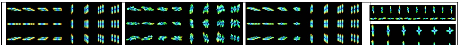
Fig. 1. Median filtering in synthetic data. From left to right: original data, noise data, filtered data.
