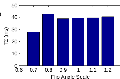
Fig. 3 T2 values with different flip angle scales.
