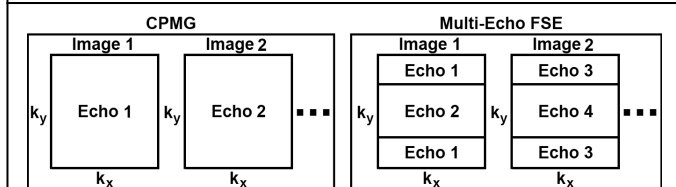
Fig. 2. Corresponding k-space of (left) CPMG and (right) centric k-space reordering of the FSE sequence with TF=2.
