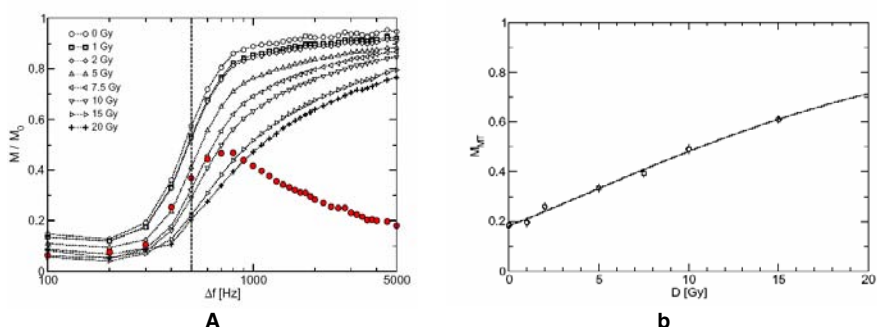
Figure 1. (a) Magnetization transfer as a function of the offset frequency of the saturation pulses for gel foam samples irradiated to different doses. A difference curve of the 0 Gy and 20 Gy sample is also shown. A dose-MT response curve is shown in (b) obtained at a saturation pulse offset frequency of 500 Hz.
