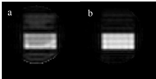
Fig. 2: (a) Pattern excited by conventional design; (b) pattern excited by joint design, which effectively adjusts phase encoding (Fig. 1) to reduce aliasing.
