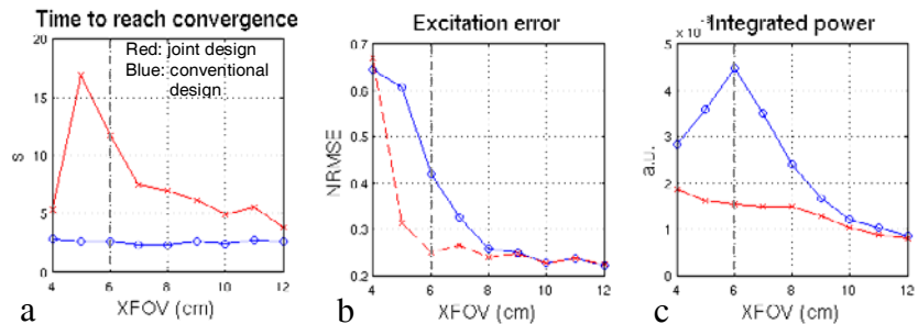
Fig. 3: In a range of acceleration factors, the joint design is beneficial in terms of excitation accuracy and pulse power, at modest computation cost. (a) Computation time for 99.9% convergence in the design methods; (b) mean square excitation error in ROI; (c) total integrated power of the eight pulses. (dash line: measures corresponding to Fig. 1 and 2)
