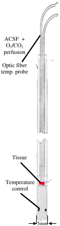
Figure 1: The MRI tissue chamber
