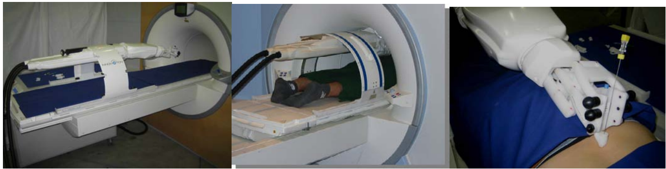
Fig. 1a, b, c: (a) INNOMOTION 6 DOF assist system (b) set up for MRI guided procedures (c) Application Module for manual cannula insertion
