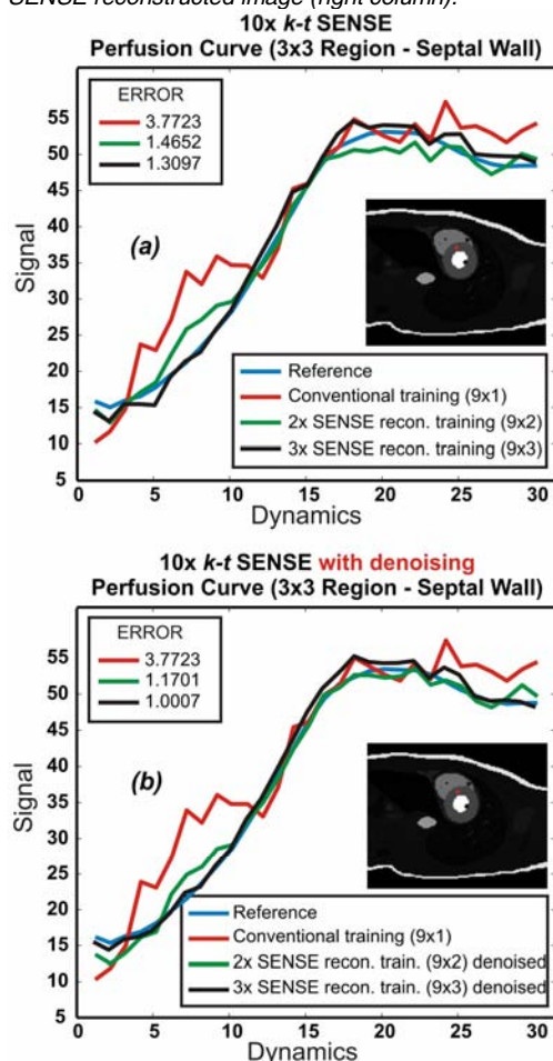
Figure 2. Upper figure: Comparison of perfusion curves from a 10x k - t SENSE reconstruction using the conventional (9 profiles) and the SENSE reconstructed training data (9x2 and 9x3 profiles undersampled by a factor of 2 and 3 respectively) along with the corresponding absolute error. Lower figure: The same comparison, this time using anisotropic diffusion filtering of the SENSE reconstructed training data.
