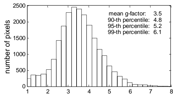
Fig 2. Histogram of SENSE g-factor for pixels in the heart volume with acceleration rate 4 \times 3=12 .
