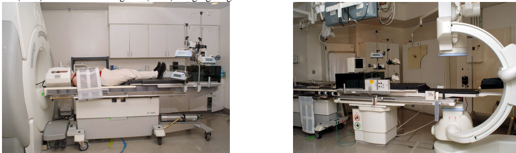
Figure 1: XMR patient transport and imaging table docked to the MR side (left) and to the X-ray angiography side (right). The transparent use of the table as a patient transport from the intensive care unit or emergency area with a full complement of MR compatible life support equipment docking to either an MR or an X-ray angiography system as an imaging platform (see Figure 1) is another key advantage of the design.
