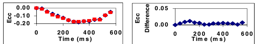
Figure 2. Plots of Ecc as a function time (left): non-accelerated (red square) and TSENSE (blue diamond). The magnitude of difference in Ecc (right).
