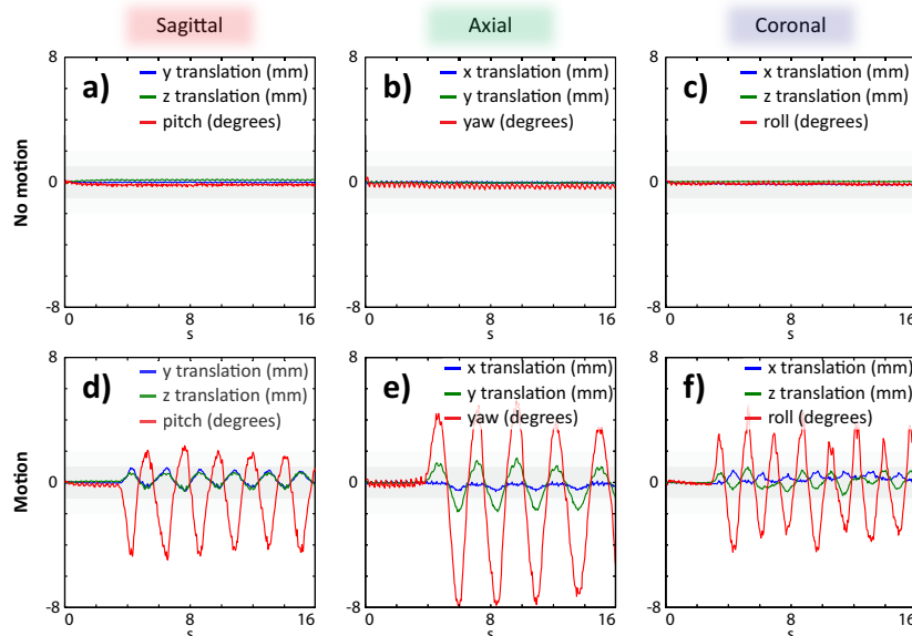
Figure 3 Motion estimates from the four experiments. No motion in the a) sagittal plane, b) axial plane, and c) coronal plane. d) pitch in the sagittal plane, e) yaw in the axial plane, and f) roll in the coronal plane.
